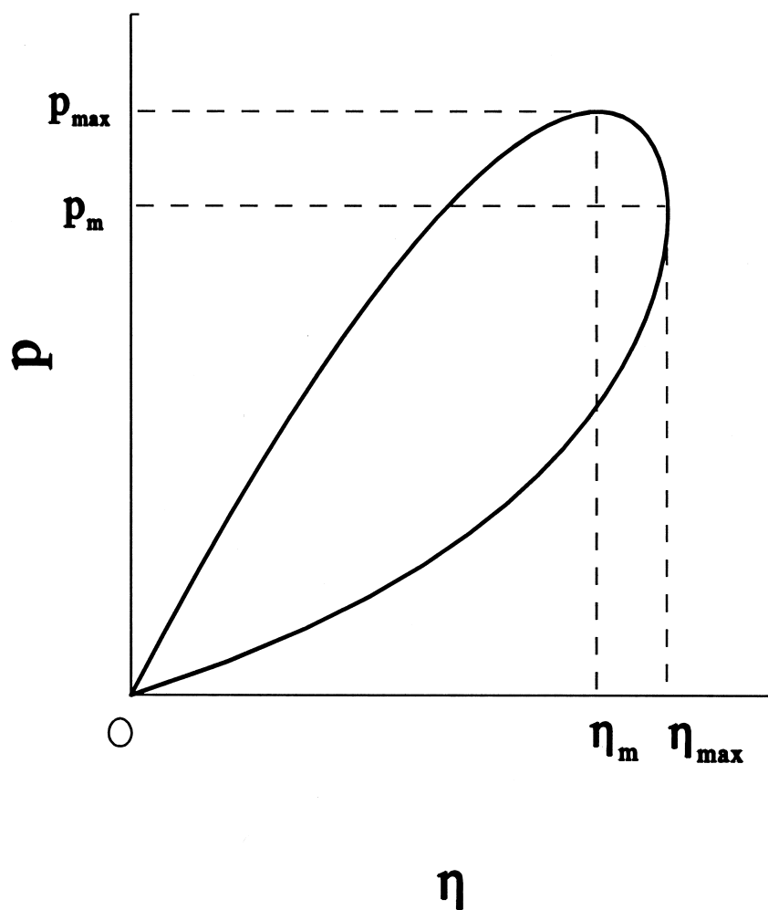
Fig. 2. The dimensionless power output versus efficiency curve of a Carnot heat engine affected by finite rate heat transfer and heat leak loss. P_{max} is the dimensionless maximum power output and P_m is the dimensionless power output at maximum efficiency \eta_{max} .
