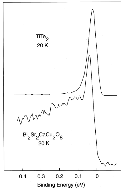
Figure 2. Photoelectron spectra of \text{Bi}_2\text{Sr}_2\text{CaCu}_2\text{O}_8 and \text{TiTe}_2 . These spectra were taken at comparable energy and angle resolutions and photon fluxes. The peak count rate for \text{TiTe}_2 is about 20 times that of \text{Bi}_2\text{Sr}_2\text{CaCu}_2\text{O}_8 . The rising edge in the \text{Bi}_2\text{Sr}_2\text{CaCu}_2\text{O}_8 spectrum is shifted away from the Fermi level because the sample is superconducting.
