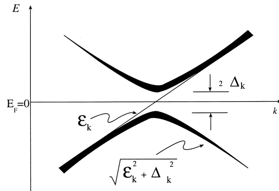
Figure 7. Behaviour of expected quasiparticle dispersion in the normal (thin straight line) and superconducting state. The line width of the lower curve for the superconducting state indicates the intensity expected in the photoelectron spectrum. (Campuzano et al., 1996).
